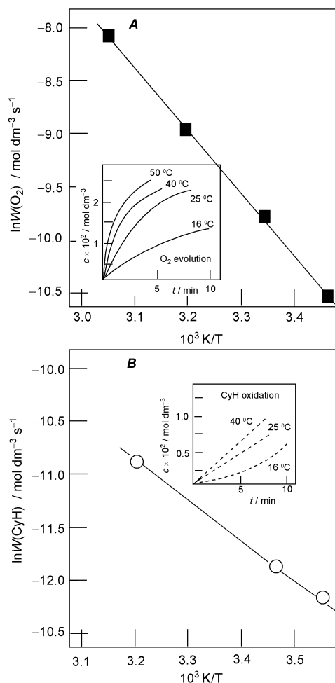
Fig. 6 Dependence of the O_2 evolution rate W(O_2) (graph A) and the cyclohexane oxygenation rate W(CyH) (graph B) on temperature. Conditions: cyclohexane (0.46 mol dm -3 ), 1a ( 5 \times 10^{-5} mol dm -3 ), H_2O_2 (0.25 mol dm -3 ), CH_3CO_2H (0.05 mol dm -3 ). Curves of dioxygen evolution and oxygenate accumulation with time at various temperatures are shown in the insets. Initial rates of these reactions are plotted in the main graphs.
